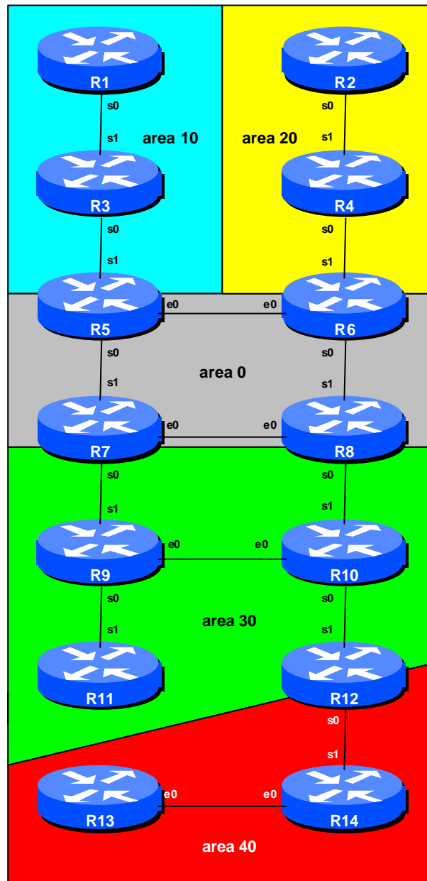
Figure 1 – OSPF Areas
