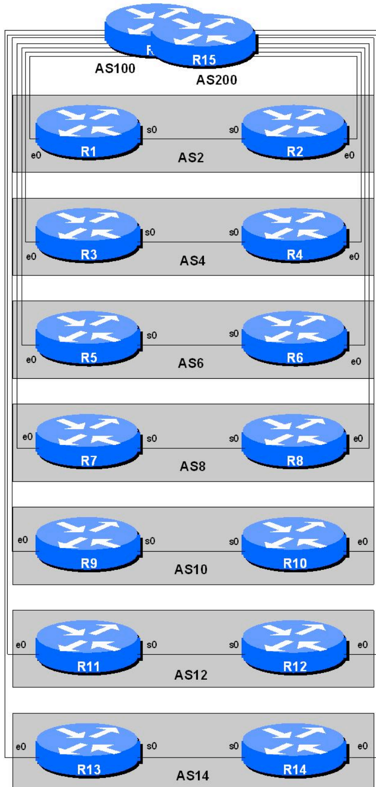
Figure 3 - iBGP and eBGP
